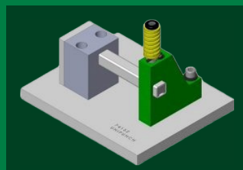
MANDREL TUBE PUNCHING UNIT
